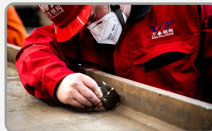
Throat Thickness Checking
